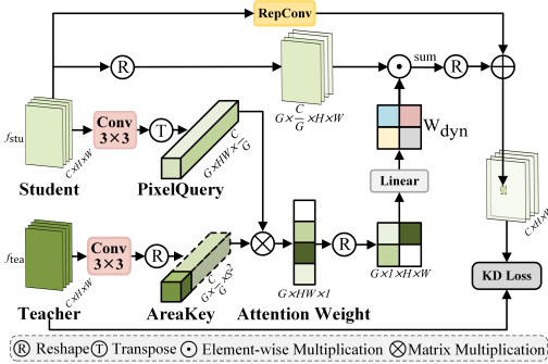
Fig. 5: Overview of our APKD.
