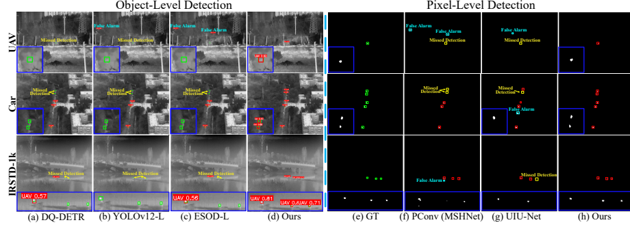
Fig. 6: Qualitative comparisons between our ECFNet and other SOTA methods on the UAV, Car and IRSTD-1k dataset. The green and red boxes denote the GT and the detection results. Closed-up views are shown in the left bottom corner and bottom.
