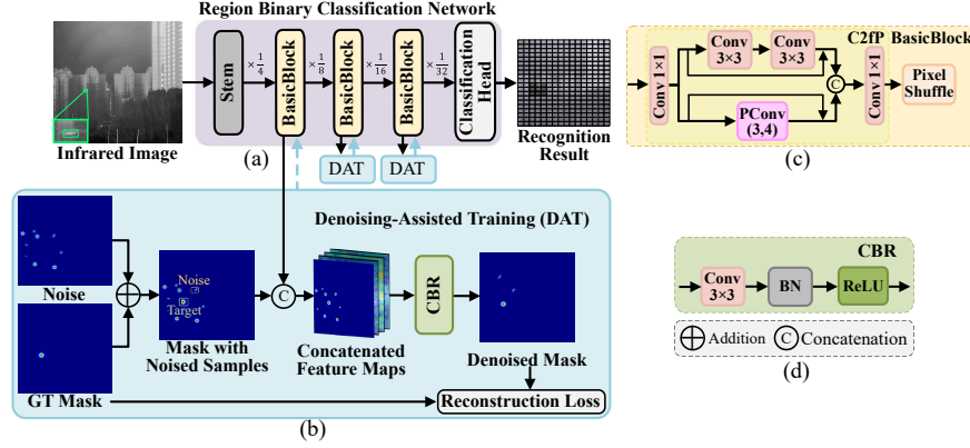
Fig. 3: Details of DAT. Multi-scale denoising prediction and GT are utilized for loss calculation. C2fP BasicBlock is a C2f-style module that mainly fuses a two-3×3-conv residual path with a PConv residual path. CBR denotes the Conv–BN–ReLU block. PConv(3, 4) [38] means the first PConv kernel is 3 and the second is 4.
