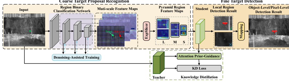
Fig. 2: The overall pipeline of ECFNet. ECFNet first employs the RBCN to generate context region proposals in the feature domain, followed by slicing these regions into square patches using the ExpSlicer. We leverage the DAT to further enhance the ability of RBCN to distinguish target proposals from complex backgrounds. In the fine stage, we customize a lightweight object-level or pixel-level detector in conjunction with an attention prior-guided knowledge distillation strategy to achieve more precise localization. Finally, we map the local region detection result back to the original image.
