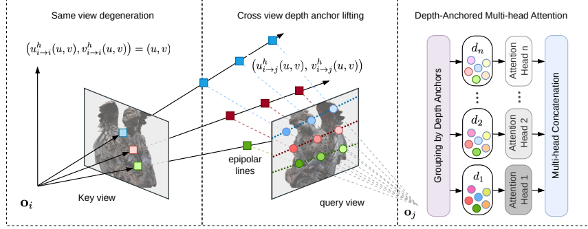
Fig. 2: Overview of URoPE. Left: URoPE reduces to standard 2D RoPE in same-view case. Middle: for cross-view interaction, a key-view pixel is lifted along its camera ray to multiple anchored depths and projected into the query view, producing anchor-specific positions along epipolar lines. Right: projected positions are assigned to different attention heads according to depth anchors as depth-anchored multi-head attention.
