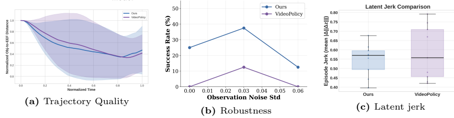
Fig. 5: Analysis. (a) Normalized object-to-end-effector distance over time. Our method shows consistent purposeful behavior and lower variance, (b) Success rate (%) under increasing observation noise. Our method maintains significantly higher performance across all noise levels, demonstrating robust semantic representations. (c) RoboTALES produces smoother latent dynamics with lower jerk, indicating more temporally coherent representations that translate to smoother robot actions.
