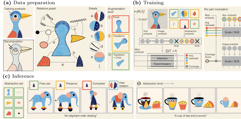
Fig. 3: Method Overview. We extract a visual abstraction set comprising disjoint elements and inter-relation details from real training images, which undergo varying levels of geometric augmentation (a). During training, we fine-tune a flow model by passing these augmented elements into a DiT alongside standard text and image embeddings; each augmentation type dictates a learned residual vector that modulates its corresponding abstraction embedding, while a global coverage score modulates the image embeddings (b). Finally, during inference, the user can define the specific generative role of individual abstraction elements (e.g., free use, preserve, or complete) and adjust the overall abstraction level to constrain the model’s expressiveness (c).
