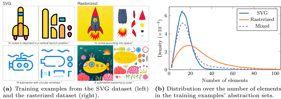
Fig. 2: FlowLess dataset mixture. Our training examples includes pairs of images and corresponding decomposed elements derived from both SVG vector images and raster images (a). The number of elements varies across different samples; SVG images tend to consist of lower number of elements (b).
