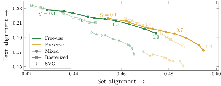
Fig. 5: Quantitative analysis. We compare the results of our method when varying coverage scores, dataset mixes, and abstraction set condition type.
