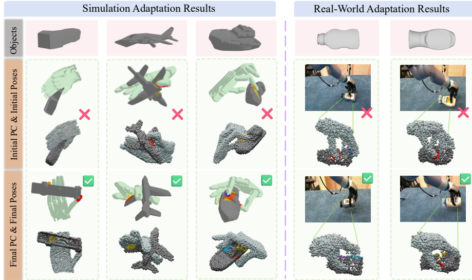
Fig. 5: Visualization of Dexterous Grasp Pose Adaptation. Row 1 presents object samples in both simulation and the real world. As shown in Row 2 (hand-object interaction mesh) and Row 3 (hand-object interaction point cloud), the initially generated grasp poses may fail to securely grasp the object, as evidenced by sparse or weak contact regions that lead to loose or unstable grasps. Row 4 and Row 5 illustrate the refined grasp poses and updated contact states after adaptation, where hand-object interaction becomes significantly more stable, with denser contact regions and a larger support area in the point cloud. These observations further validate the effectiveness of the proposed adaptation module in correcting suboptimal initial grasps.
