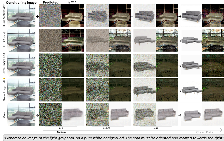
Fig. 4: Internal representations. We visualize both the predicted image and the decoded conditioning latent \mathbf{h}_L^{\text{cond}} at different timesteps during denoising. Model evaluated without fine-tuning: (i) FLUX.1 Kontext [dev] [26]; (ii) FLUX.2 [dev] [5]; (iii) Qwen-Image-Edit-2509-Lightning [33] and (iv) Qwen-Image-Edit-2509 [52]. We also visualize our method’s internal representation after fine-tuning. FLUX models maintain representations of the conditioning image throughout denoising, whereas Qwen models encode the final prediction in \mathbf{h}_L^{\text{cond}} even at high noise levels ( t \approx 1 ). Note that our method encodes the prediction in the embedding space while preserving the original geometry.
