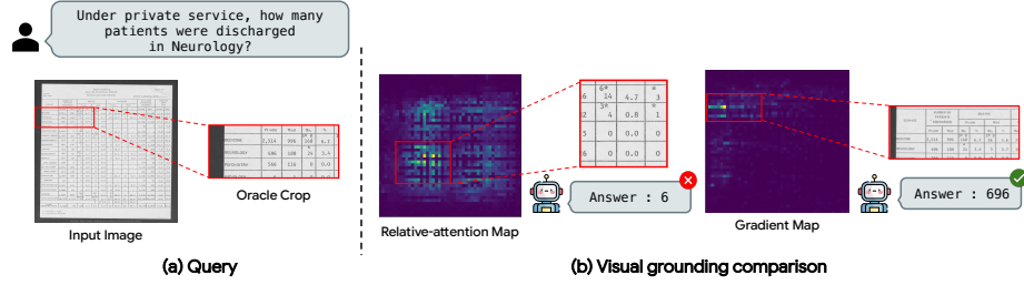
Fig. 3: Relative attention vs. entropy-gradient. Given an image and a user query as shown in (a), we compare the attention-based grounding used in ViCrop [42] with our proposed entropy-gradient grounding in (b). The relative-attention map produces a diffuse heatmap that highlights an incorrect region, leading to a wrong crop and an erroneous answer (6). In contrast, the entropy-gradient map concentrates on the query-relevant row of the table, yielding a precise crop that enables the model to correctly answer the question (696).
