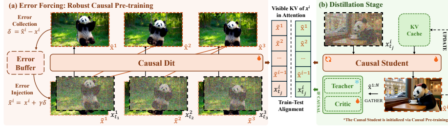
Fig. 3: Illustration of our overall pipeline. (a) We first employ the Error Forcing paradigm, proactively degrading the ground-truth (GT) context via error injection to construct an error-aware, robust causal pre-trained model. (b) Subsequently, we bypass the conventional ODE-based adaptation and directly apply distillation for few-step generation. Benefiting from Error Forcing, train-test consistency is inherently satisfied during distillation.
