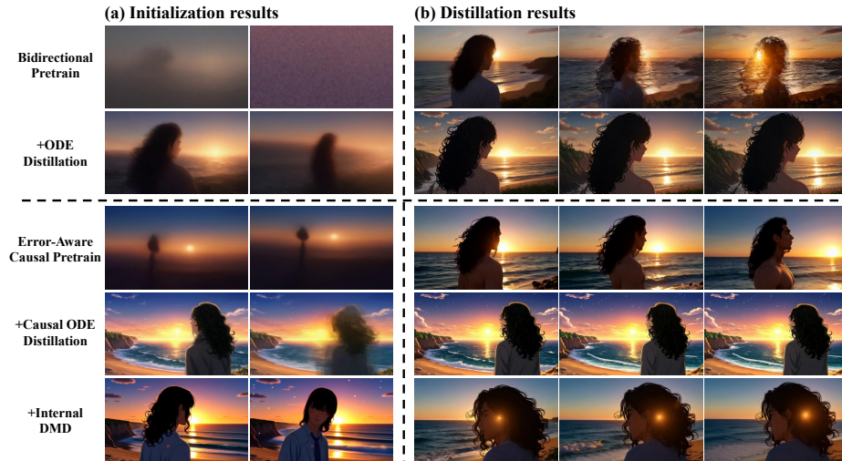
Fig. 7: Qualitative comparison of different initializations. (a) Few-step inference results of various bidirectional and causal initializations before distillation. Note that Internal DMD employs an architecturally identical teacher and critic to solely distill the few-step capability. (b) Corresponding results after external model (Wan2.1-T2V-14B) distillation.
