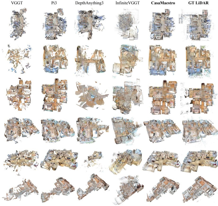
Fig. 5: Quantitative comparison on Realsee-Real.
