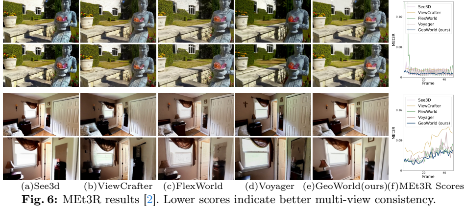
Fig. 6: MET3R results [2]. Lower scores indicate better multi-view consistency.
