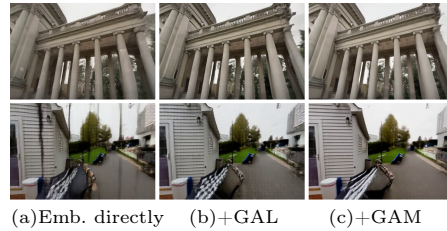
Fig. 10: Visual comparisons of the design of the geometry-constrained diffusion model. ‘GAL’: geometric alignment loss. ‘GAM’: geometry adaptation module.
