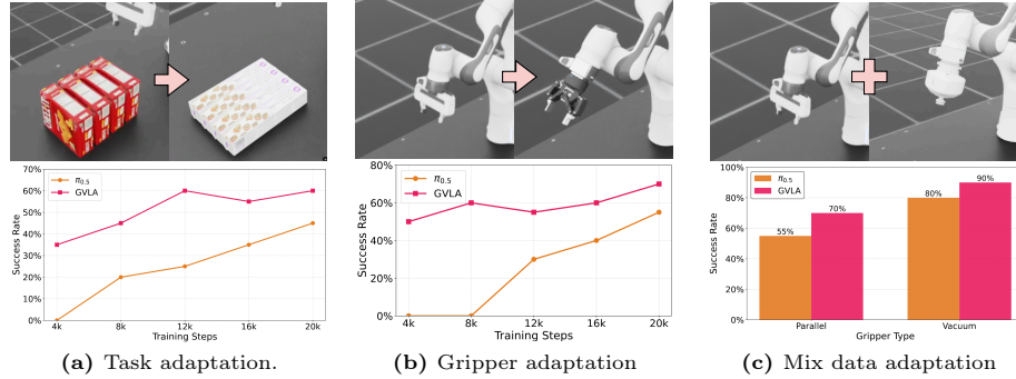
Fig. 9: Adaptation results.
