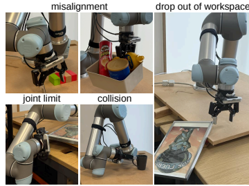
Fig. 11: Failure cases
