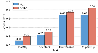
(b) Cross-object generalization success rate.
