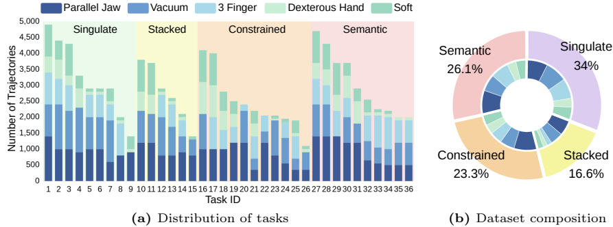
Fig. 4: MiGA dataset statistics.
