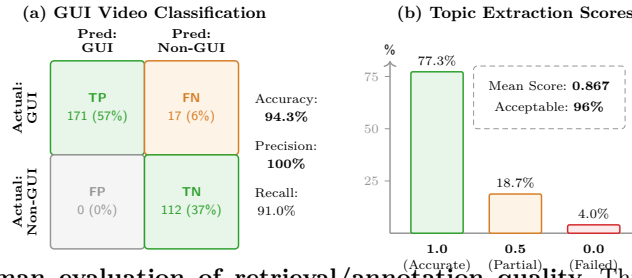
Fig. 5: Human evaluation of retrieval/annotation quality. Three annotators score 300 videos per stage: (a) GUI classification keeps 100% precision; (b) topic extraction reaches mean 0.867 and 96% acceptable.
