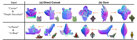
Fig. 11: Normal map comparison at fusion boundary. Direct Concatenation exhibits sharp discontinuities, whereas ours produces smoother normals across the fusion region.
