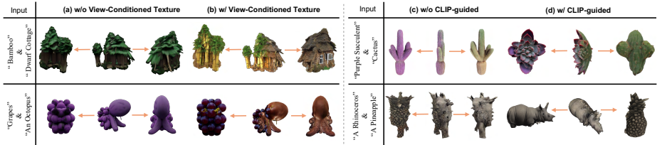
Fig. 16: Ablation on texture synthesis and orientation search. Each pair shows View 1, blended mesh, and View 2. (a) w/o View-Conditioned Texture : Standard texturing fails on fused geometries, blending semantics into indistinguishable appearances (e.g., uniform foliage or solid purple). (b) w/ View-Conditioned Texture (Ours) : Accurately assigns distinct, prompt-driven textures to each viewpoint. (c) w/o CLIP-guided : Fixed 0^\circ/180^\circ angles cause silhouette misalignments, failing to reveal clear semantics. (d) w/ CLIP-guided (Ours) : Adaptive rotation optimally aligns silhouettes, recovering distinct semantics at both views.
