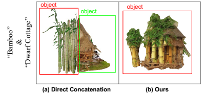
Fig. 8: Object detection at the junction viewpoint for “Bamboo” & “Dwarf Cottage”. (a) Direct Concatenation is detected as two separate objects (red and green boxes); (b) Ours is detected as a single unified object (red box only).
