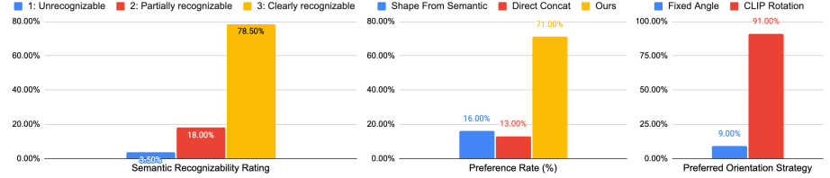
Fig. 12: User study. (Left) Semantic Recognizability: 78.5% of participants rated our results as clearly recognizable (score 3). (Middle) Method Preference: 71% of participants preferred our method over Shape From Semantics [38] (16%) and Direct Concatenation (13%). (Right) Orientation Strategy: 91% of participants found CLIP-guided orientation to produce a more natural illusion than fixed 0°/180° angles.
