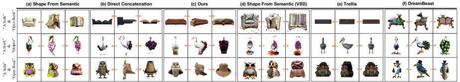
Fig. 9: Qualitative comparison with baselines. Left-to-right: View 1, blended mesh, View 2. (a) Shape From Semantics [38] suffers from over-saturation and geometry leakage. (b) Direct Concatenation exposes unnatural junction seams and opposing geometry at target views. (c) Ours produces a coherent mesh with clear, view-dependent semantics and no leakage. (d) Shape From Semantics (VSD) [38] still exhibits over-saturation and leakage despite its stronger objective. (e) TRELLIS [71], prompted with “a single 3D object, front side is A, back side is B”, fails to produce view-dependent semantics and collapses to a generic shape that reflects neither target interpretation. (f) DreamBeast [40] blends both semantics uniformly across all viewpoints, failing to achieve view-dependent separation.
