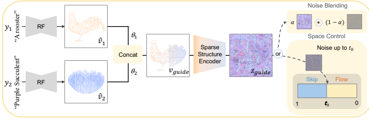
Fig. 5: Noise Guidance. Given two prompts y_1 and y_2 , two single-semantic voxels \hat{v}_1 and \hat{v}_2 are independently generated and concatenated at \theta_1 and \theta_2 to form v_{\text{guide}} , encoded into z_{\text{guide}} via the Sparse Structure Encoder. Noise Blending Guidance mixes z_{\text{guide}} with pure noise via \alpha \cdot z_{\text{guide}} + (1 - \alpha) \cdot z_{\text{noise}} , injecting a mild spatial prior. Space Control Guidance interpolates between z_{\text{guide}} and noise at timestep t_0 , providing stronger structural constraints for geometrically challenging pairs.
