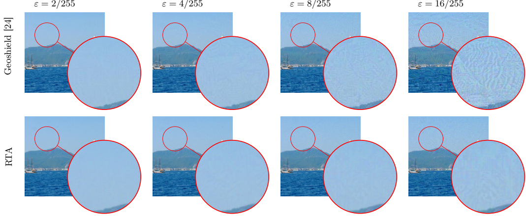
Fig. 2: Visual comparison of adversarial noise for four budgets \varepsilon = 2/255, 4/255, 8/255, 16/255 and two methods (Geoshield and ours). The magnified area highlights the fine-grained perturbation patterns for the attack. Best viewed in color on a screen.
