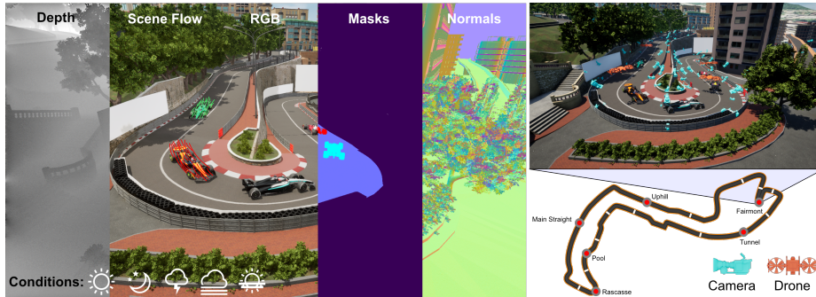
Fig. 2: Overview of the Monaco4D benchmark.: We cover six sections of the Monaco circuit with dense multi-view camera coverage, multimodal ground-truth annotations (RGB, depth, normals, masks, scene flow), under five illumination conditions.
