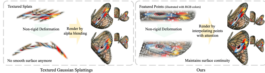
Fig. 2: Comparison of geometry deformations of textured Gaussian splatting methods and PointGT. Left: Since each Gaussian is a linear primitive, these methods struggle to preserve surface smoothness under large non-rigid deformations. Right: PointGT maintains surface continuity after deformation by predicting ray-surface points via attention-based interpolation on a point cloud.
