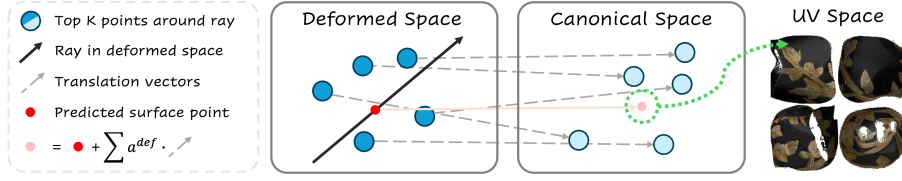
Fig. 3: Illustration of the deformation-aware canonical correspondence. In deformed space (left), a ray intersects the deformed point cloud to predict a surface point (red). Each deformed neighbor (dark blue) has a stored canonical counterpart (light blue); the per-neighbor displacements (dashed gray arrow) are fused with the deformed-space attention weights to transfer the intersection back to canonical space (middle), where UV lookup retrieves the texture (right).
