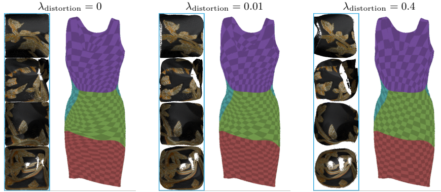
Fig. 8: Learned UV mapping under different weights of the proposed distortion loss.
