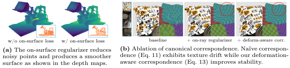
Fig. 7: Ablation studies on geometry regularization and canonical correspondence.
