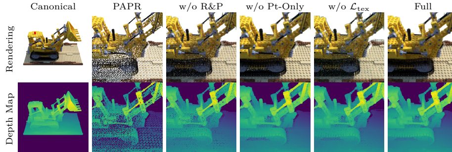
Fig. 6: Ablation study on the Lego scene under 2\times scaling. From left to right: canonical (undeformed), vanilla PAPR, without rays-and-points (R&P) mode, without points-only mode, without texture loss \mathcal{L}_{\text{tex}} , and our full pipeline.
