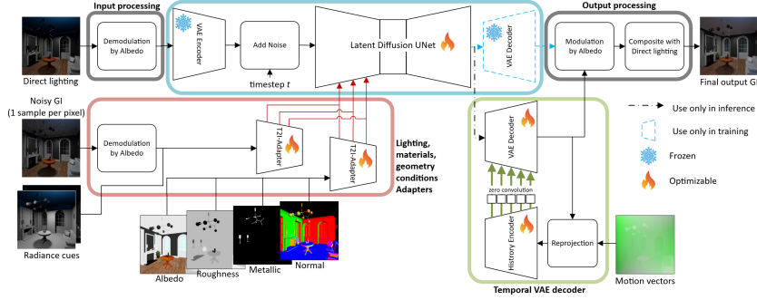
Fig. 1: Overview of our method. Given an initial lighting hint from direct lighting, our approach generates global illumination using a conditional one-step diffusion model. Multiple conditioning inputs are encoded via adapter modules and injected into the diffusion model. We use geometry (normals), material properties (albedo, roughness, metallic), and lighting cues (direct lighting, spatially sparse GI, radiance cues) as conditioning inputs. The proposed Temporal VAE decoder ensures temporal consistency over long sequences. We train the Temporal VAE decoder separately and replace the frozen VAE decoder with it at inference time. A diagram of TVAE training appears in the supplementary material.
