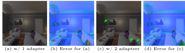
Fig. 10: Ablation of using two adapters, which produces better indirect lighting. The error maps are produced by CGVQM [24].
