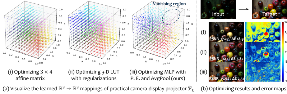
Fig. 5: Effectiveness of the Learned Model for \hat{\mathcal{F}}_{\mathbf{C}}(\cdot; \theta) . In contrast to an affine fit (i) or a learned 3D LUT [57] (ii), our model (iii): captures (a) higher-frequency details and (b) achieves better performance. Notably, the learned projector exhibits a “vanishing” region where multiple camera color collapse to the same displayed color.
