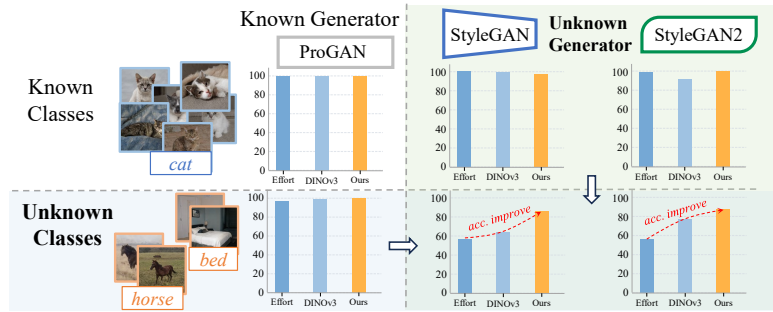
Fig. 1: Semantic Bias in VFM-based Detection. Detectors trained exclusively on Cat images are evaluated on both seen and unseen semantic classes. Baseline methods (Effort [83], LoRA-tuned [24] DINOv3 [65]) suffer a severe performance drop on novel semantics, revealing a heavy reliance on semantic cues rather than actual forgery patterns. In contrast, our BCNet corrects the decision basis to focus on intrinsic synthesis traces, achieving robust semantic generalization across diverse categories.
