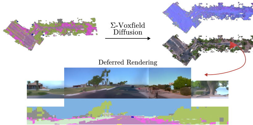
Fig. 1: Our model generates large-scale 3D driving scenes given a coarse semantic voxel grid. Here we show a generated large-scale driving scene spanning \approx 100\,000 m 2
