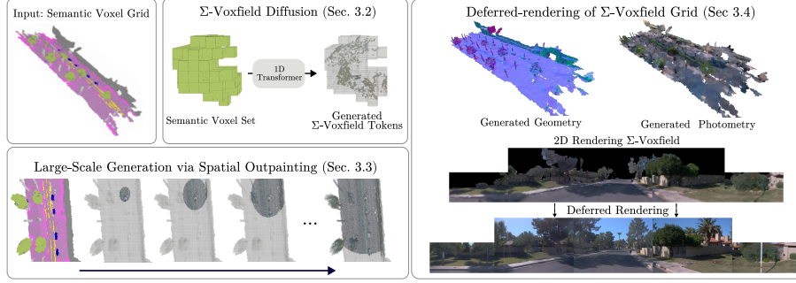
Fig. 2: Overview of SEM-ROVER. Our framework performs generation directly in 3D to ensure consistent geometry and appearance. It represents the scene with a \Sigma -Voxfield grid and applies transformer-based diffusion over 3D tokens. To scale to large environments efficiently, we use an iterative outpainting strategy. Finally, a deferred rendering engine converts the generated 3D scene into photorealistic views.
