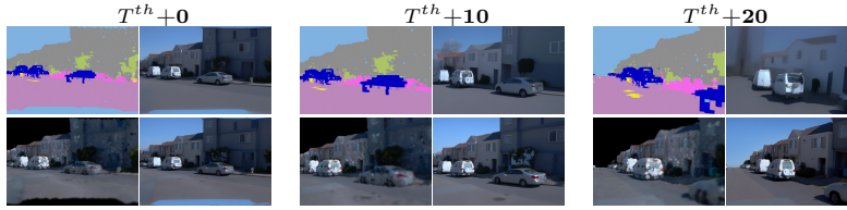
Fig. 8: Comparison of \Sigma -Voxfield (bottom) vs semantic field (top) conditioning for ASD-based rendering
