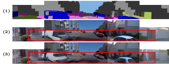
Fig. 10: Scene inpainting We mask a voxel region as shows (1) (darker voxel colors for unmasked) and re-generate only this region while keeping the rest of the \Sigma -Voxfield grid fixed. (2) and (3) show two inpainted results (red box) that remain coherent with the background and vary in both structure and appearance.
