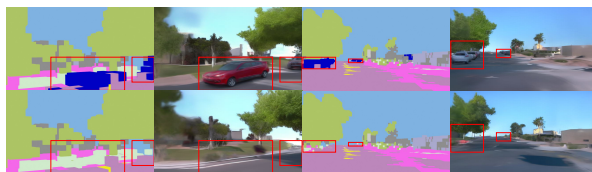
Fig. 9: Semantic editing: We remove existing cars by editing the semantic grid (red boxes), then regenerate the content conditioned on the updated semantics. The generated results remain coherent and consistent with the surrounding scene.
