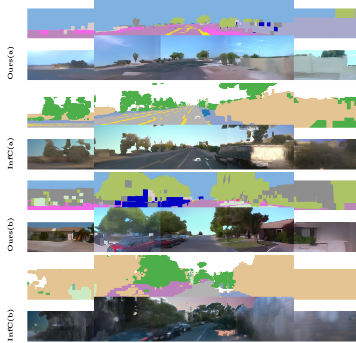
Fig. 6: Qualitative comparison to InfiniCube [15]. For two waymo scenes (a) and (b), we show five camera of the semantic conditioning and below the rendered generated scenes for Our method (Ours) and Infincube (InfC).
