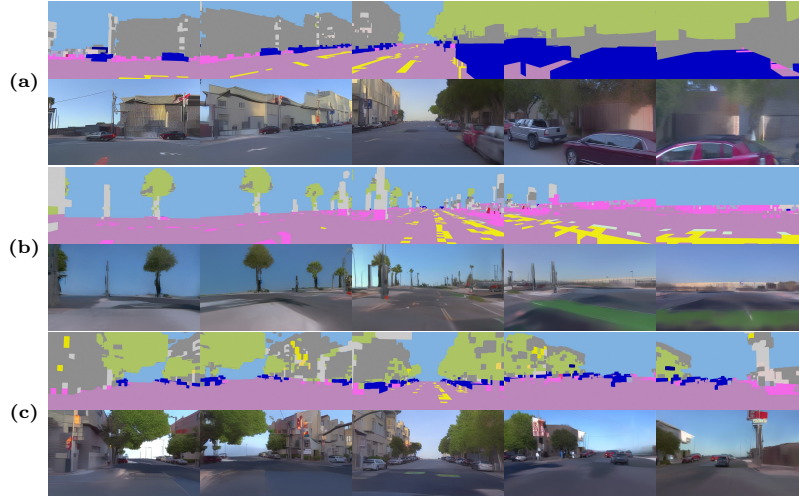
Fig. 5: Qualitative results on PandaSet. We show three PandaSet scenes (a–c). For each scene, the top strip visualizes the semantic voxel rendering used for conditioning, and the bottom strip shows the corresponding generated scene from 5 camera views.
